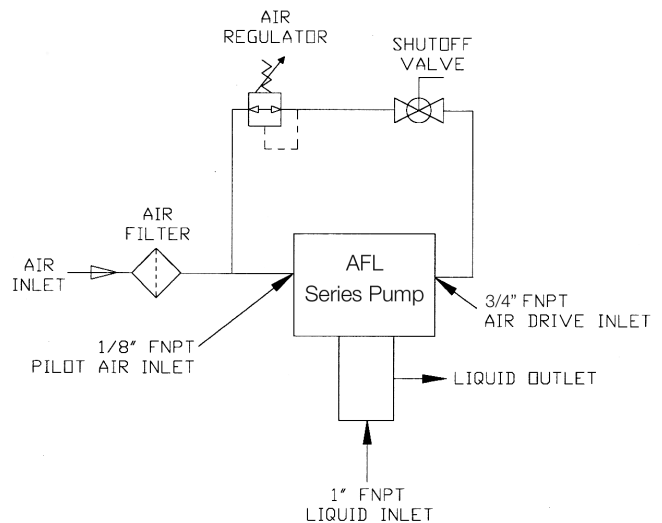
Air Line Schematic
